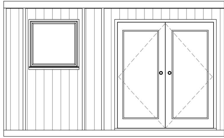
2 Front Elevation 1 : 40
